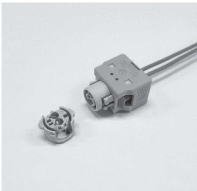
Shunt-less Squib Connector. Connector for air-bag with Go/No-Go system, which allows locking connector and detect incomplete mating.
