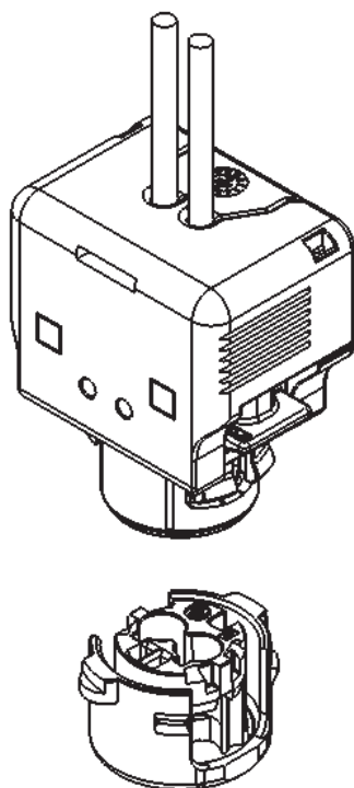
Shunt-less Squib Connector. Connector for air-bag with Go/No-Go system, which allows locking connector and detect incomplete mating.
