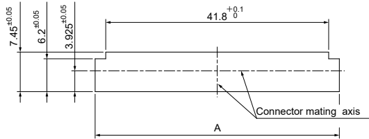
Recommended panel dimensions
