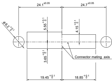
Recommended panel dimensions (Panel thickness : 1.2mm)
