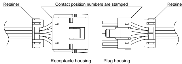
Receptacle housing
